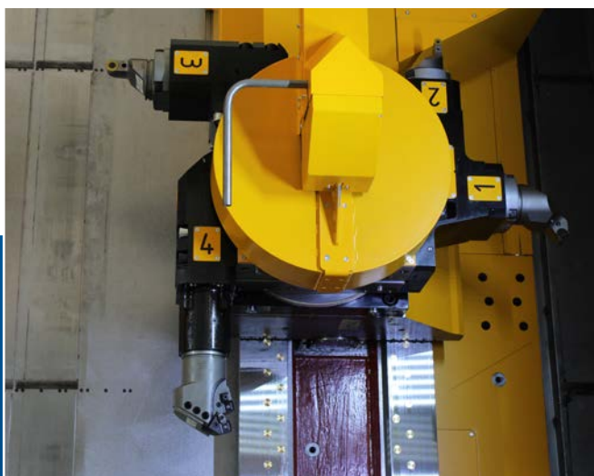
REVOLVER HEAD
