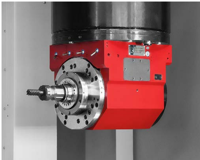
HORIZONTAL ELECTROSPINDLE
