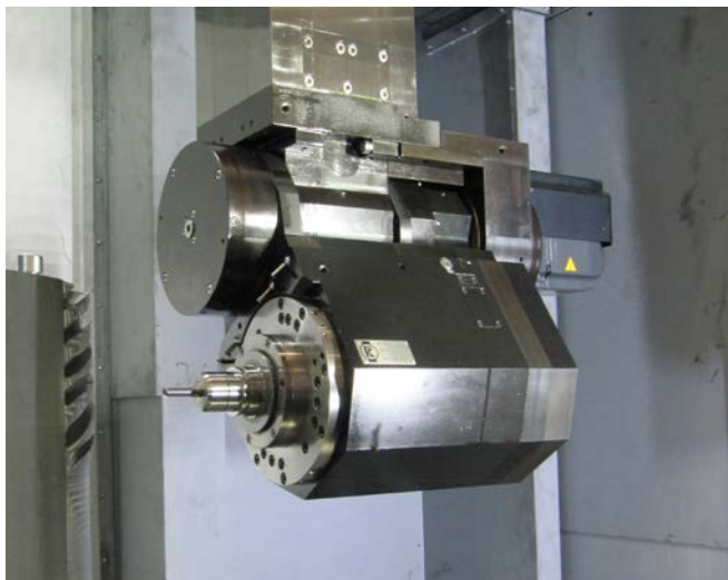
Y-HEAD
