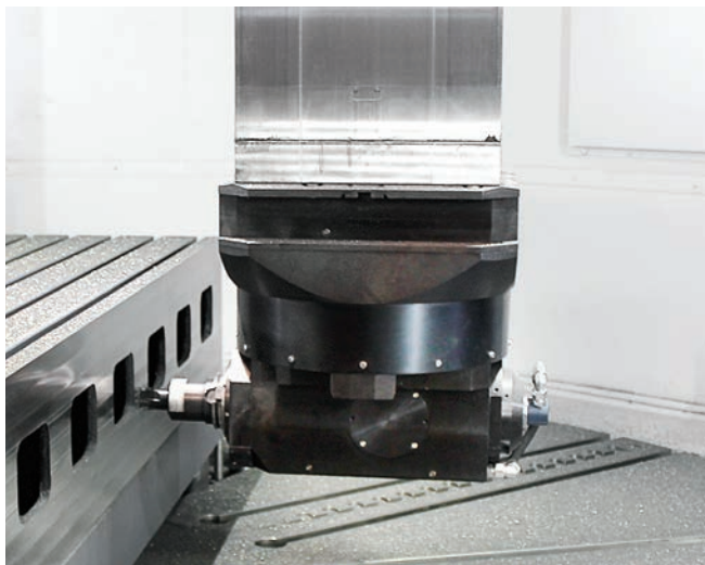
C-HEAD
