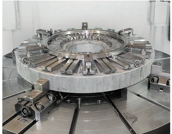
MAGNETIC TABLE
